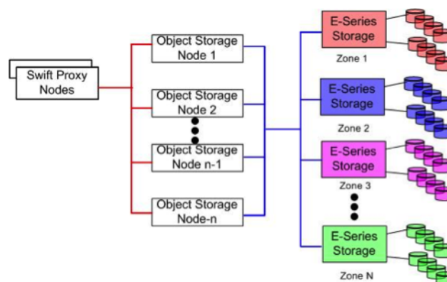
Figure 7.2. Controller-subsystem based zoning
