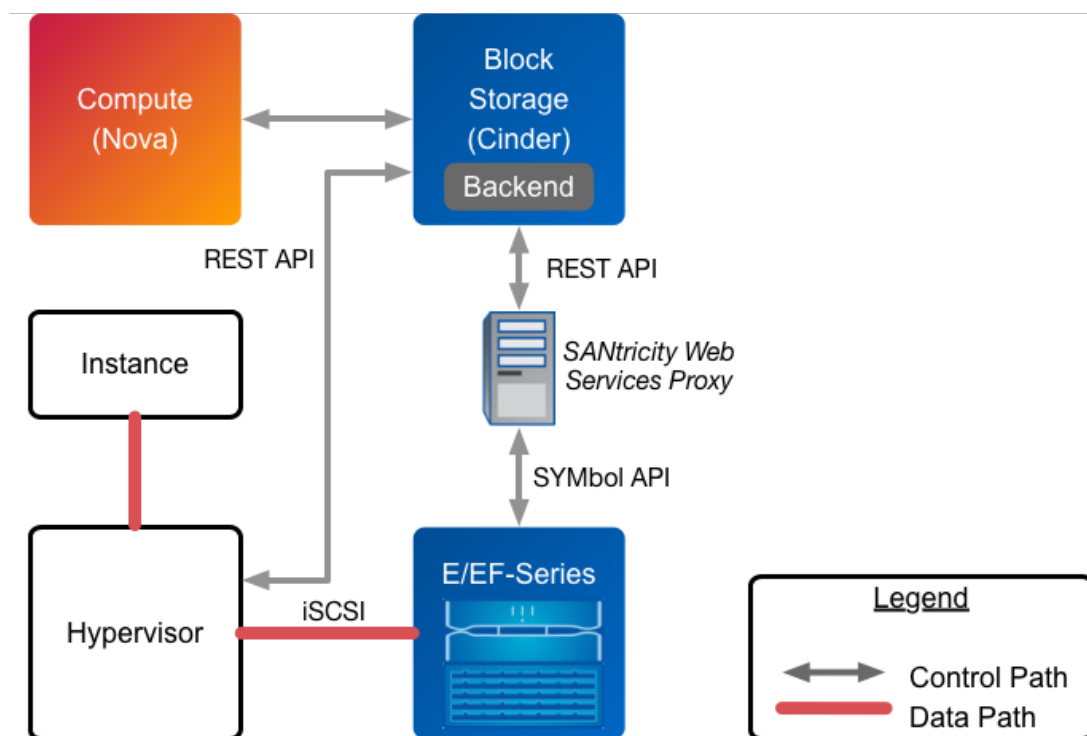
Figure 4.5. Cinder & E-Series Deployment Topology
